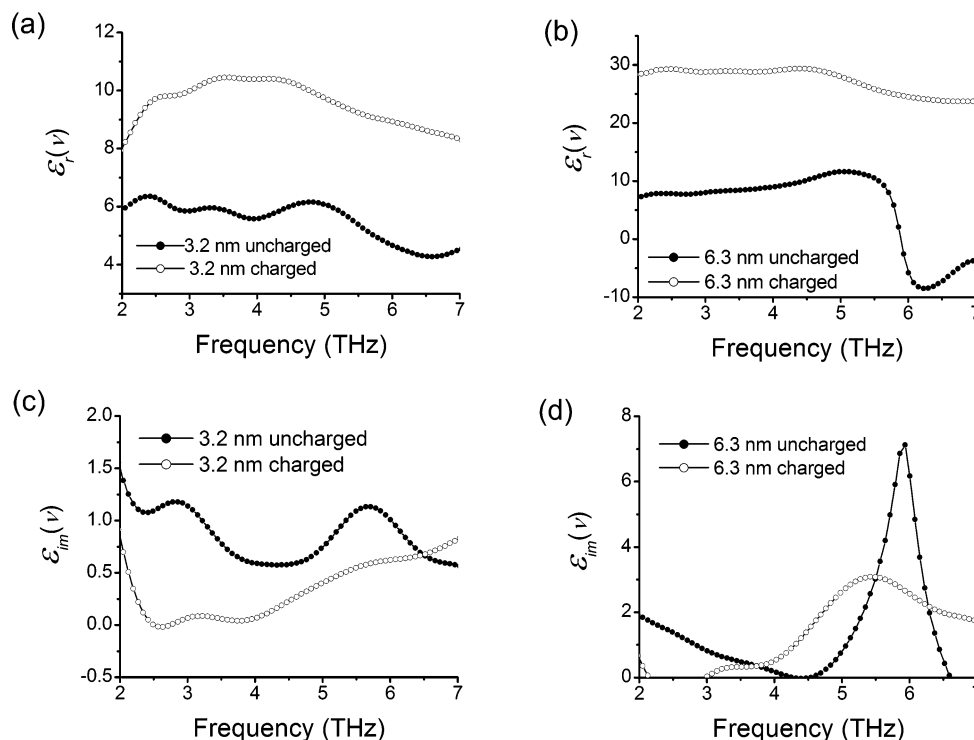
Figure 5. Intrinsic complex dielectric constants of the uncharged and charged quantum dots evaluated from the experimentally obtained effective dielectric constants: (a) and (b) real part and (c) and (d) imaginary part of the complex dielectric constants.
