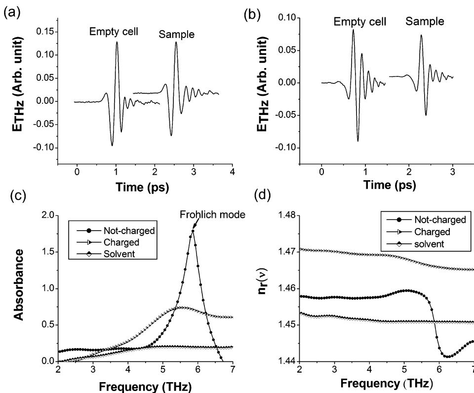
Figure 4. THz TDS measurements of the large (6.3 nm) uncharged and charged CdSe quantum dots. (a) THz waveform measured for the empty sample cell and uncharged quantum dots. (b) THz waveform measured for the empty sample cell and charged n-type quantum dots. (c) Frequency-dependent THz absorbance of the uncharged and charged quantum dots and the solvent obtained from the spectra in (a) and (b). (d) Real refractive indices of the uncharged and charged quantum dots and the solvent.
