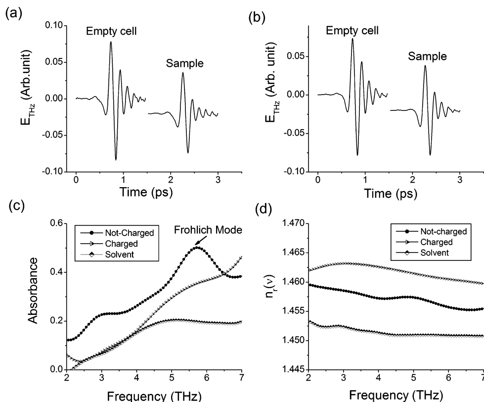
Figure 3. THz TDS measurements of the small (3.2 nm) uncharged and charged CdSe quantum dots. (a) THz waveform measured for the empty sample cell and uncharged quantum dots. (b) THz waveform measured for the empty sample cell and charged n-type quantum dots. (c) Frequency-dependent THz absorbance of the uncharged and charged quantum dots and the solvent obtained from the spectra in (a) and (b). (d) Real refractive indices of the uncharged and charged quantum dots and the solvent.
