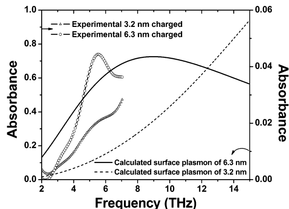
Figure 6. Calculated THz absorption spectra of the singly charged quantum dots of two different sizes due to surface plasmon from the Drude model for metal particles. The experimental THz absorbance of 3.2 and 6.3 nm charged CdSe QD solutions are also included in the plot. The experimental absorbance are about 10 times higher than the calculated surface plasmon modes.
